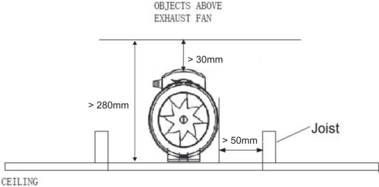
Fig.4 Clearance diagram
