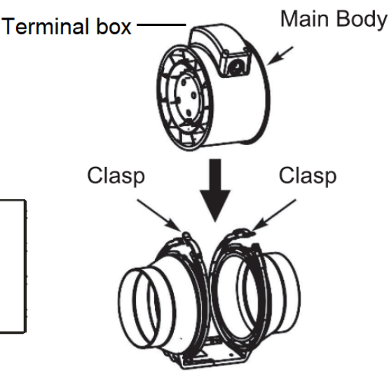
Fig. 3 – Install main body
